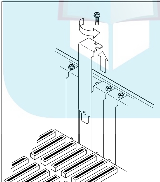
Figure 5-1: Remove the slot cover and screw before installing a new card.
